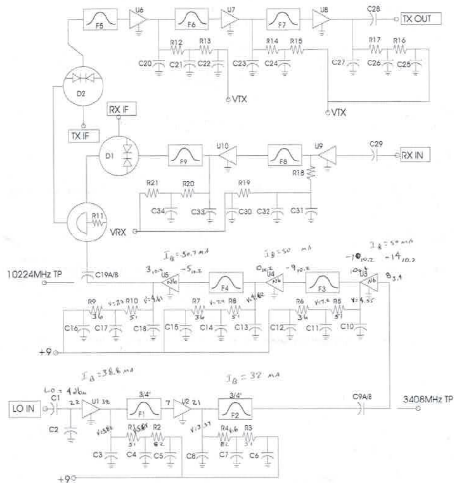
10368-144LP TRANSVERTER SCHEMATIC
