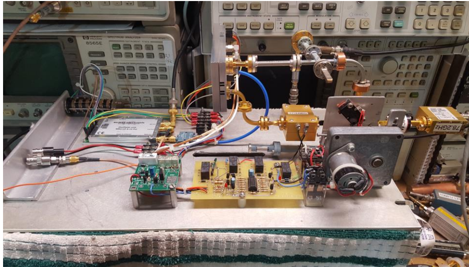
Figure 1 76GHz Transverter assembly in progress
